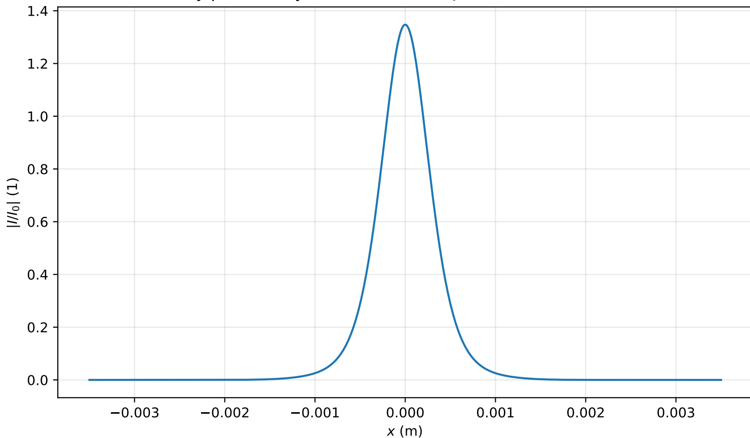
Intensity profile I(x, y = 0, z = 1.751m)/I_0 , P_{in}=0.8P_{cr} , artificial time
